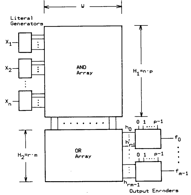
Fig. 5. p -valued PLA with output encoders (Type 2 PLA).
