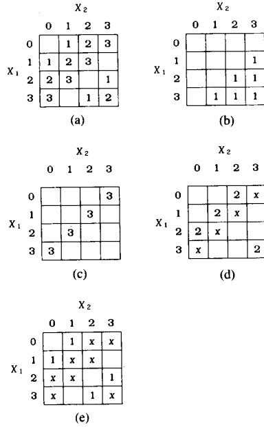
Fig. 3. Maps for adder using Type 1 PLA. (a) Sum. (b) Carry. (c) g_3 . (d) 2 \cdot g_2 . (e) 1 \cdot g_1 .
