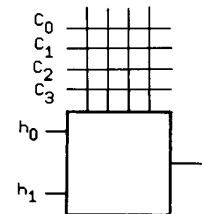
Fig. 13. Programmable output encoder (four-valued).
