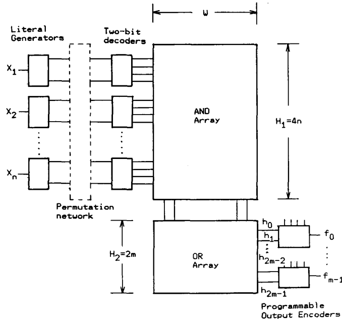
Fig. 14. Four-valued PLA with 2-bit decoders and programmable output encoders.
