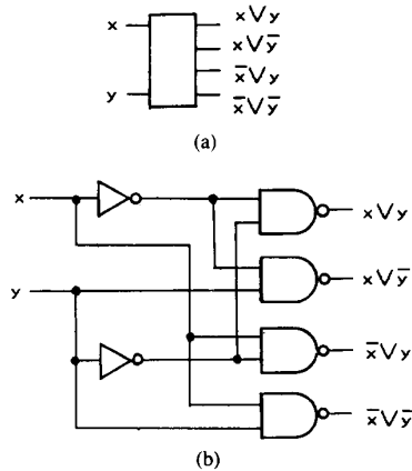
Fig. 16. 2-bit decoder. (a) Logic symbol. (b) Circuit realization.
