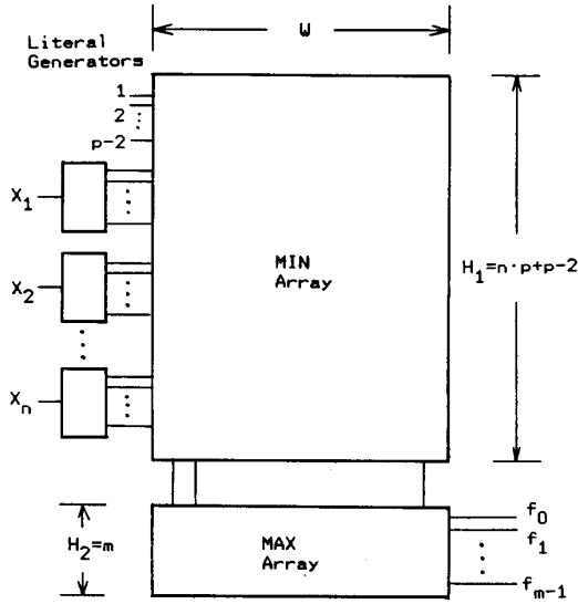
Fig. 1. p -valued PLA with MIN and MAX array (Type 1 PLA).
