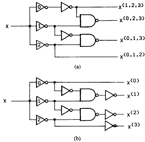
Fig. 9. Literal generator. (a) For NAND-NAND structure. (b) for NOR-NOR structure.
