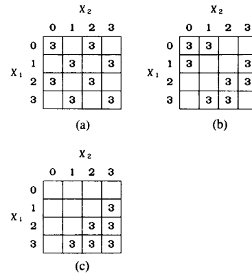
Fig. 11. Maps for adder using Type 2 with optimal output encoding. (a) h_1 . (b) h_0 . (c) C_0 .
