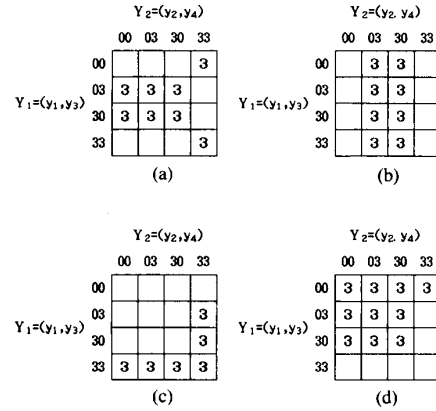
Fig. 17. Maps for adder with Type 2 PLA with 2-bit decoders. (a) S_1 . (b) S_0 . (c) C_0 . (d) C_0 .
