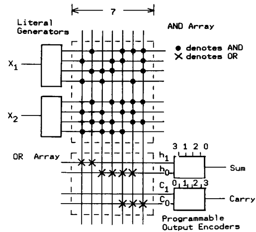
Fig. 12. Adder using Type 2 PLA with optimal output encoding.
