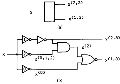
Fig. 15. Literal generator. (a) Logic symbol. (b) Circuit realization.
