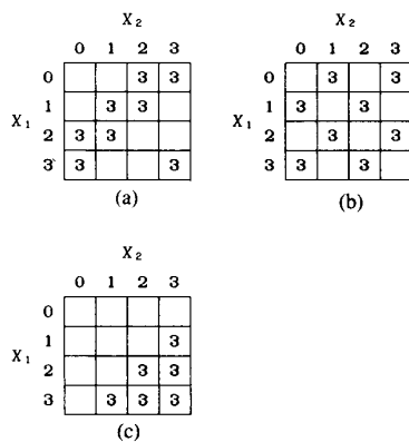
Fig. 7. Maps for adder using Type 2 PLA. (a) S_1 . (b) S_0 . (c) C_0 .
