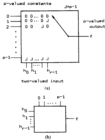
Fig. 6. Output encoder. (a) p -input multiplexer. (b) Symbol for output encoder.
