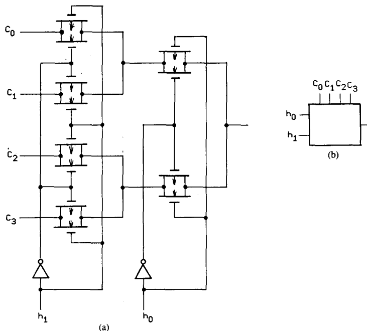
Fig. 10. Output encoder (four-valued) (a) CMOS realization. (b) Logic symbol.
