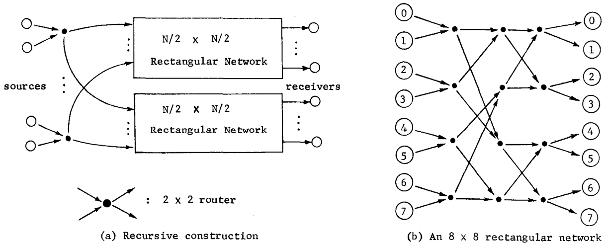
Figure 7. Rectangular Routing Network
