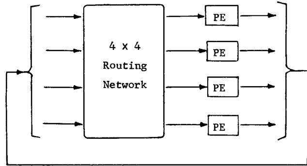
Figure 3. First data flow machine prototype.
