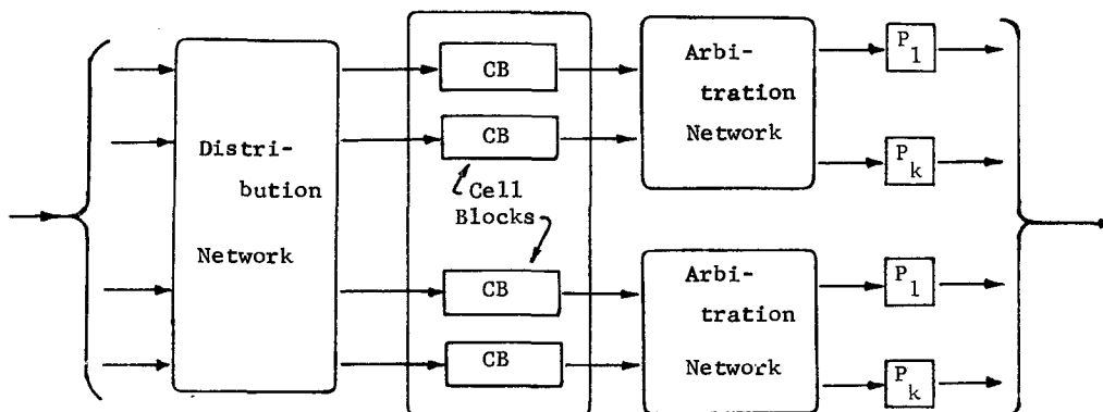
Figure 1. Data flow processor
