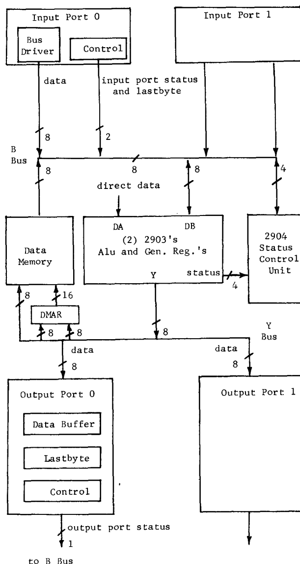
Figure 9. Data paths of the PE.
