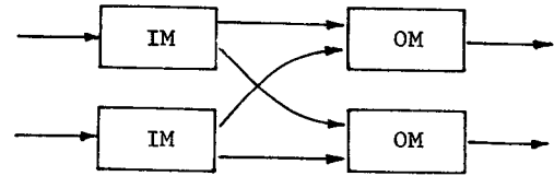
Figure 6. Structure of a router module.
