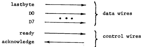
Figure 4. Hardware structure of a module connection.
