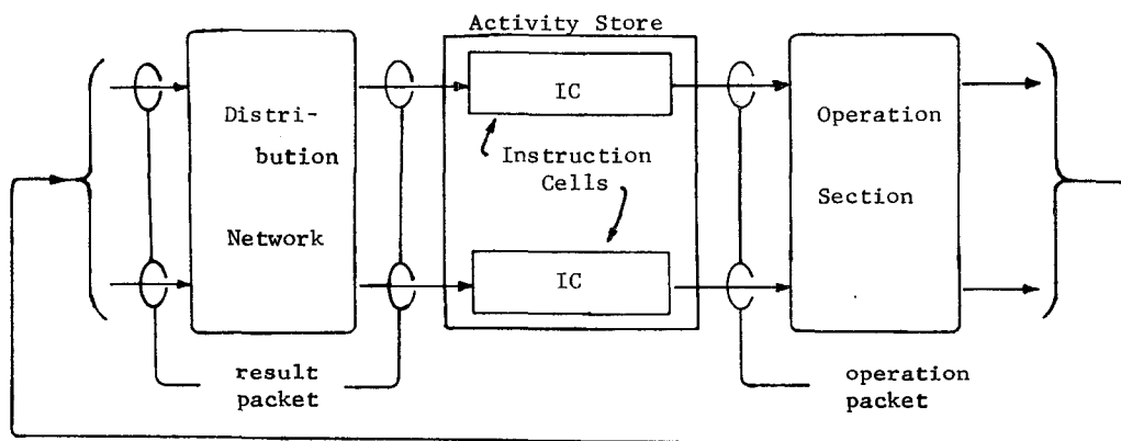
Figure 1. Data flow processor
